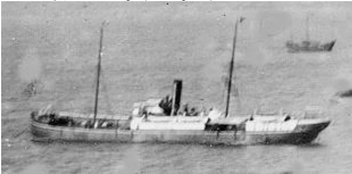
KWANGSE or a sister in Chefoo harbour (UoB Carral coll. Ca02-092).
