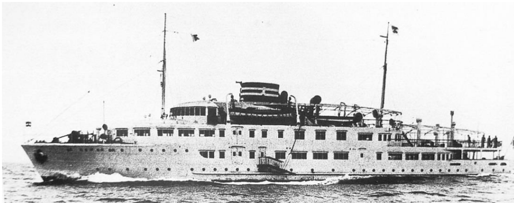
SHIROGANE MARU had no sheer and minimal camber ( Kaiun 1938).
